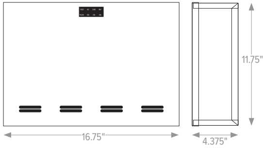
LG125T Recessed Ceiling T-Grid Mount Model
